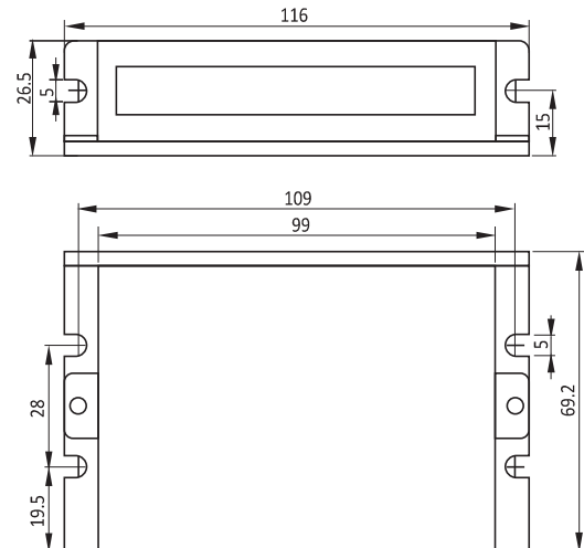
(b) Mechanical specifications of the EM503
