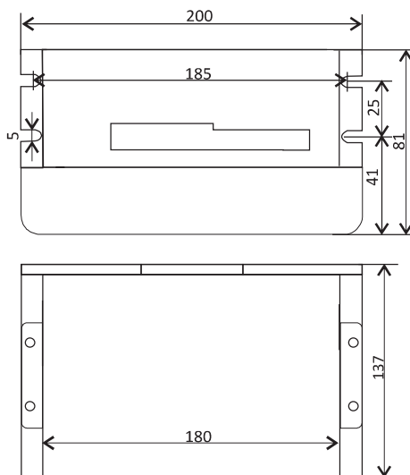
(e) Mechanical specifications of the EM1206H and EM2306H
