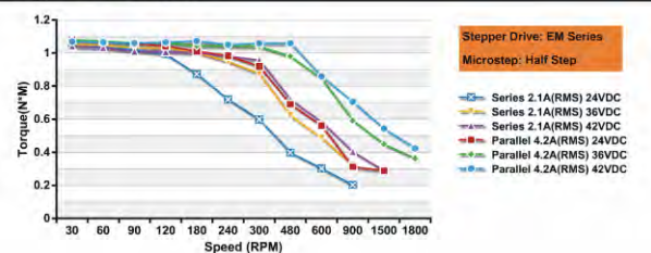
Stepper Motor: 57HS22
